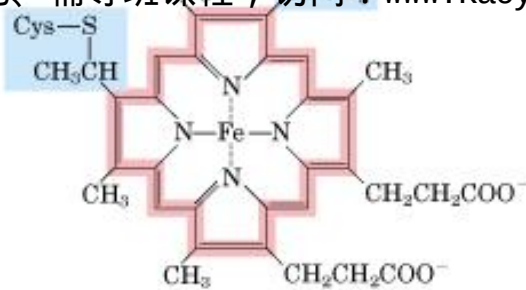
Heme C (in c -type cytochromes)
