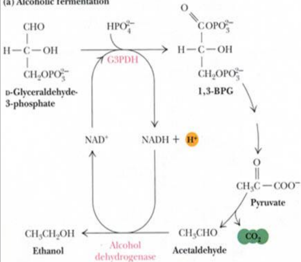
(a) Alcoholic fermentation
