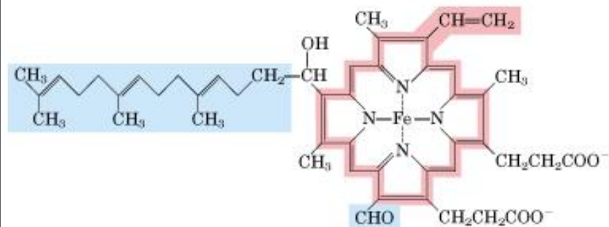
Heme A (in \alpha -type cytochromes)
