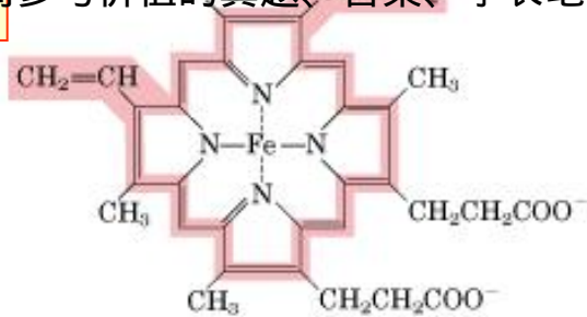
Iron protoporphyrin IX (in b -type cytochromes)
