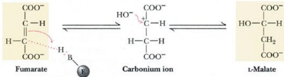
Carbonium ion mechanism
